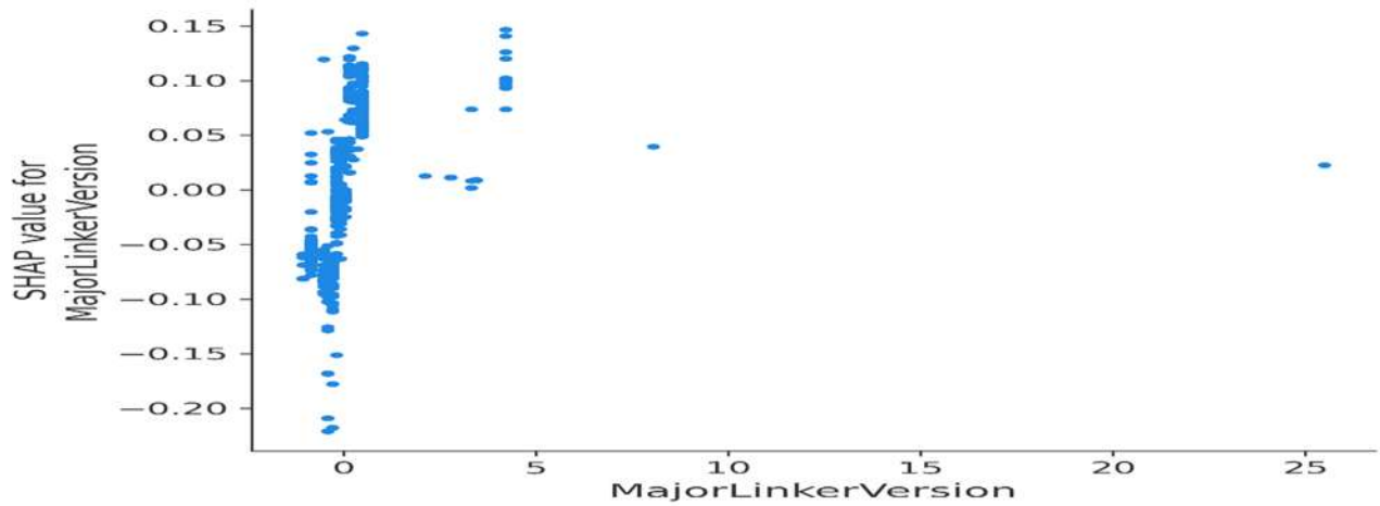
Figure 3. SHAP Dependence Plot for Major Linker Version Feature.
