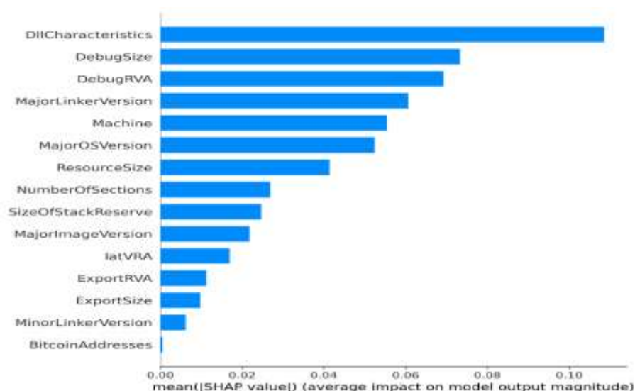
Figure 2. Global SHAP Feature Importance Analysis.
