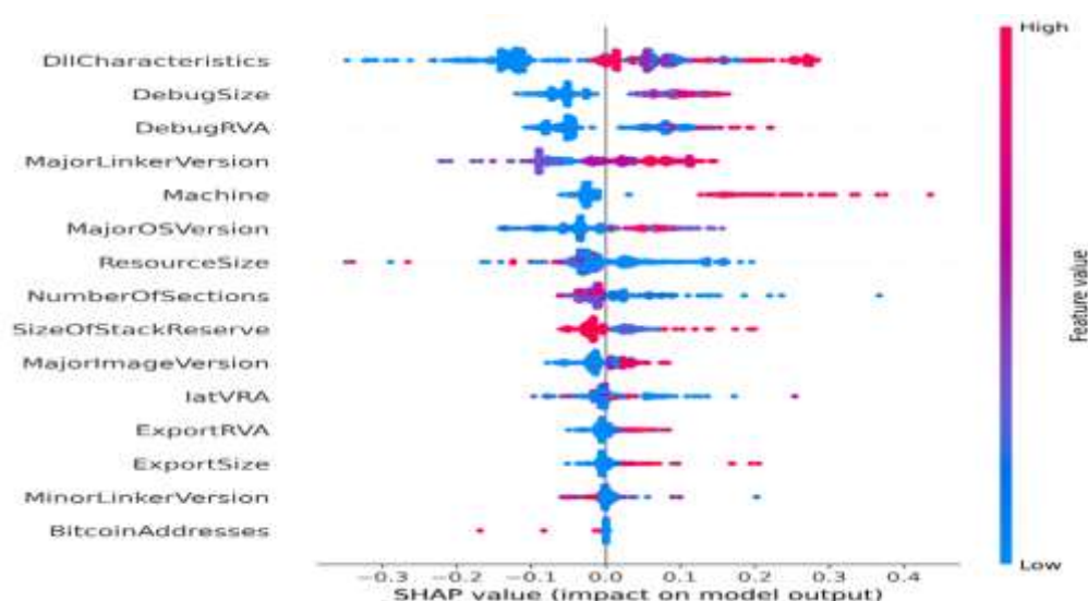
Figure 1. SHAP Summary Plot for Malware Detection Features.
