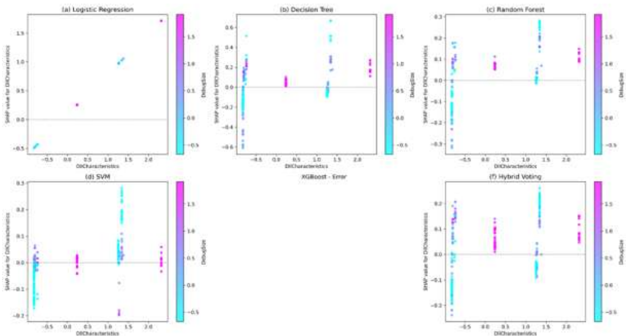
Figure 4. Comparative SHAP Analysis Across Models.
